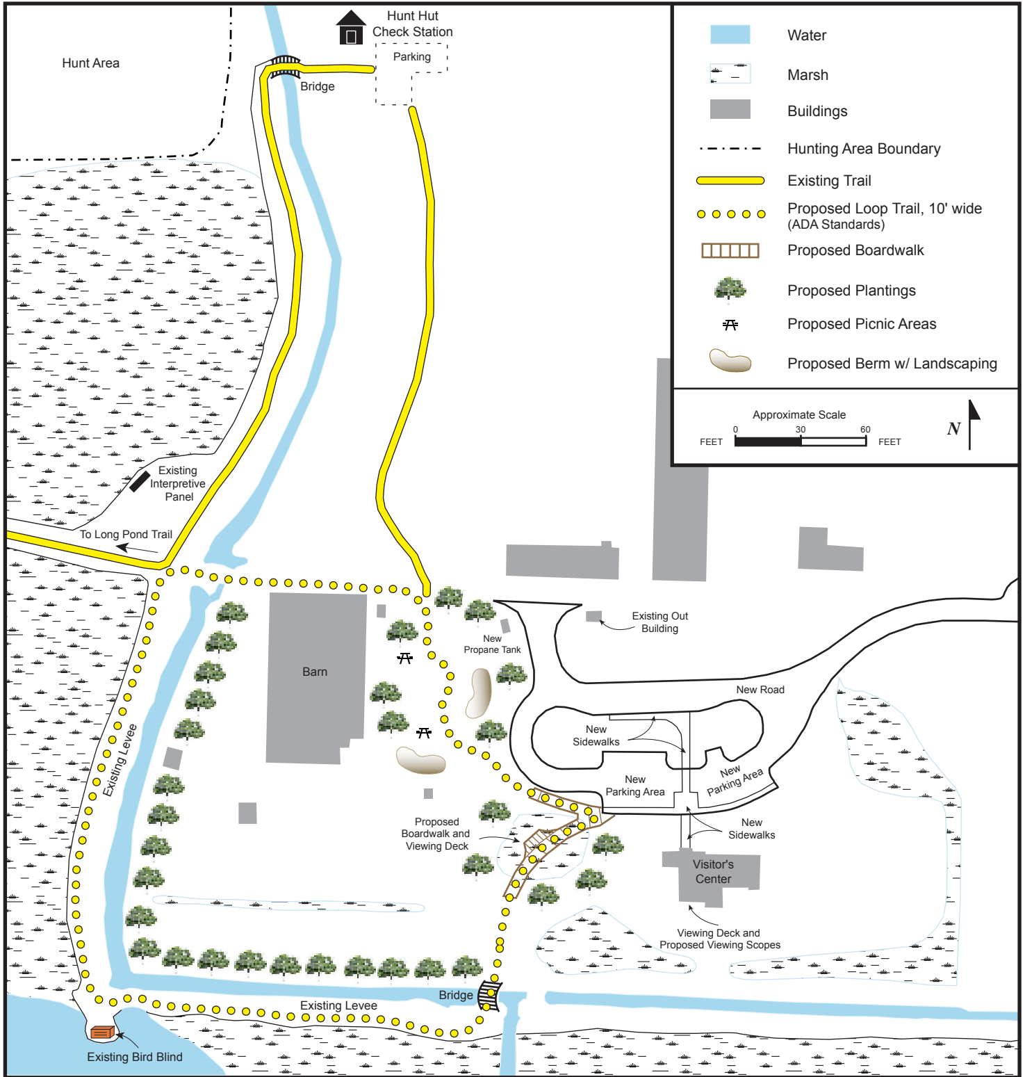
FIGURE III-9. HUMBOLDT BAY NATIONAL WILDLIFE REFUGE SOUTH BAY SYSTEM SITE PLAN
