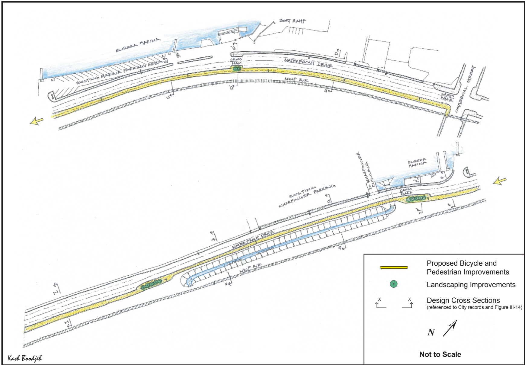
FIGURE III-15. WATERFRONT DRIVE PLAN VIEW (CONCEPTUAL)
